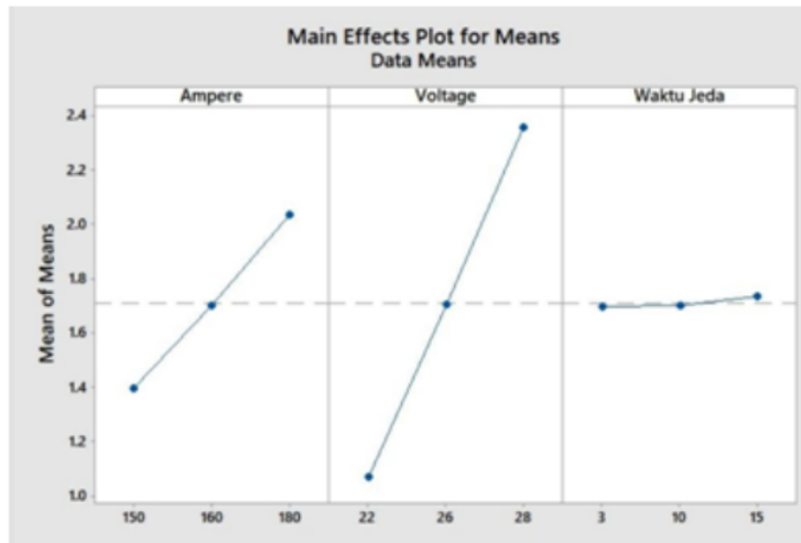
Figure 2 Effect Plot of Welding Parameters on Deformation
