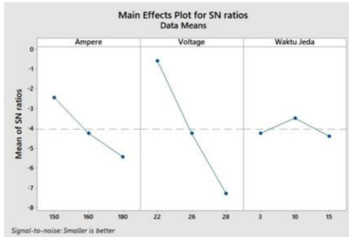
Figure 3 Plot S/N Ratio
