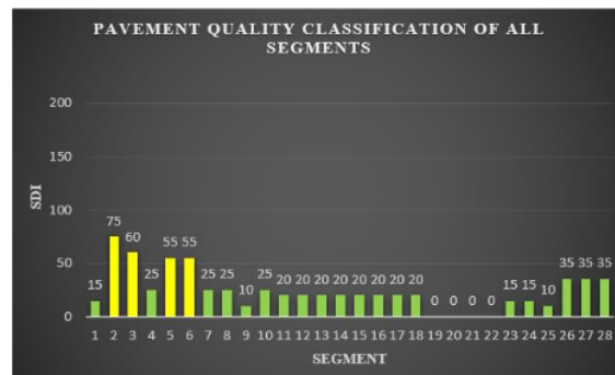
Figure 4. SDI Value Graph of the entire Segment
